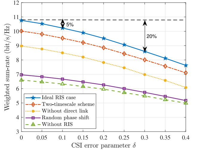
Fig. 8. Weighted sum-rate against the CSI error parameter \delta .
