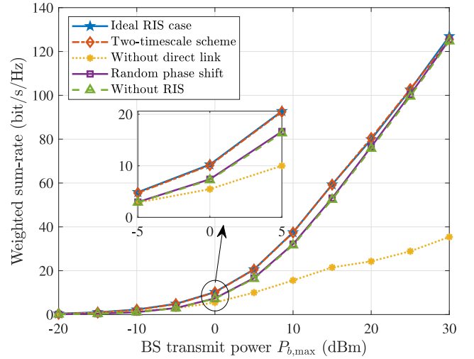
Fig. 9. Weighted sum-rate against the BS transmit power P_{b,\max} .
